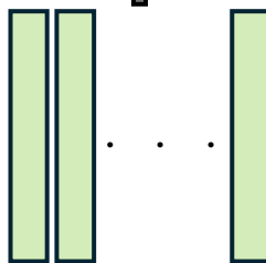
Text Features
