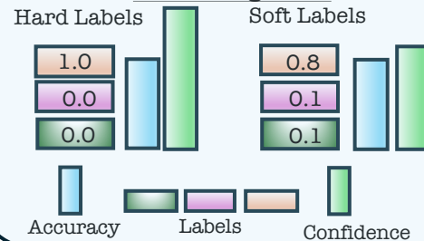
Matching Loss
